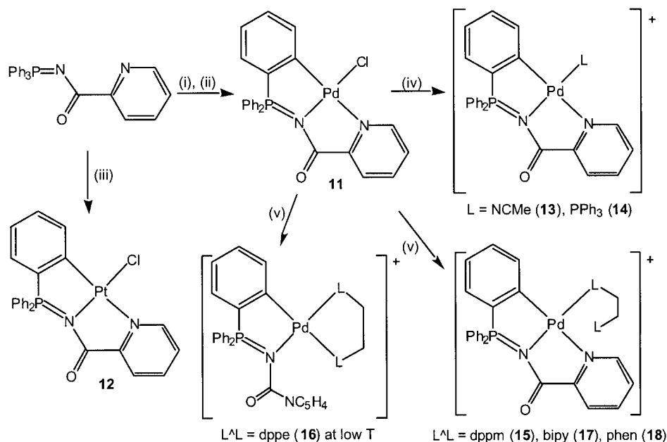
Scheme 2. (i) \text{Pd}(\text{OAc})_2 , reflux, \text{CH}_2\text{Cl}_2 ; (ii) \text{LiCl} , room temp., \text{MeOH} ; (iii) [\text{PtCl}_2(\text{NPh})_2] , 2-methoxyethanol, reflux; (iv) \text{AgClO}_4 , -\text{AgCl} , \text{L} , \text{NMe} or acetone, room temp.; v) \text{AgClO}_4 , -\text{AgCl} , \text{L} , acetone, room temp.
