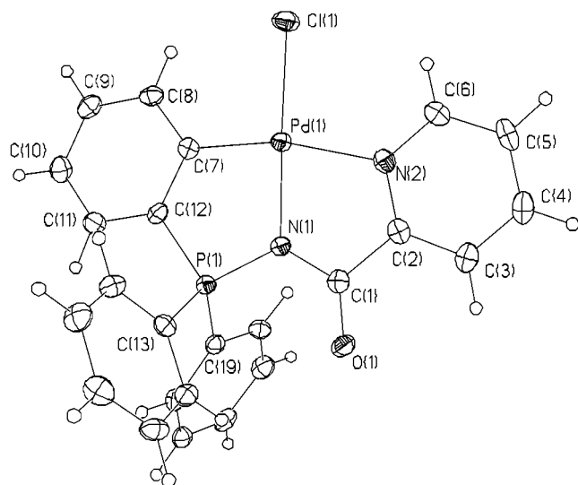
Figure 1. Thermal ellipsoid plot of [\text{Pd}(\text{C}_6\text{H}_4\text{-}2\text{-PPh}_2\text{=N-C(O)-}2\text{-NC}_5\text{H}_4\text{-}\kappa\text{-C,N,N})\text{Cl}] ( 11 ). Non-hydrogen atoms are drawn at the 50% probability level.
