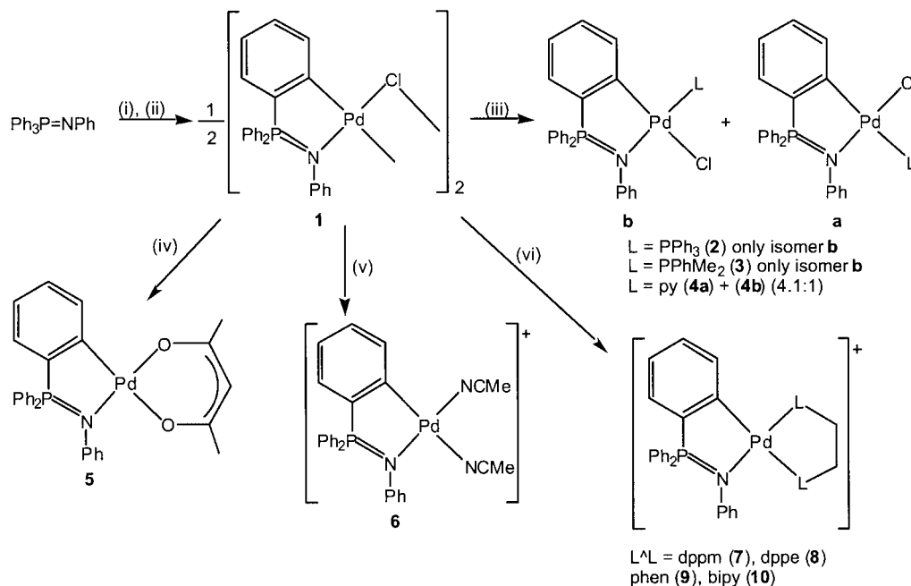
Scheme 1. (i) \text{Pd}(\text{OAc})_2 , reflux, \text{CH}_2\text{Cl}_2 ; (ii) \text{LiCl} , room temp., \text{MeOH} ; (iii) \text{L} , \text{CH}_2\text{Cl}_2 , room temp.; (iv) \text{Ti}(\text{acac})_3 , \text{TiCl}_4 , \text{CH}_2\text{Cl}_2 , room temp.; (v) \text{AgClO}_4 , \text{AgCl} , \text{NMe} , room temp.; (vi) \text{AgClO}_4 , \text{AgCl} , \text{L} , acetone, room temp.
